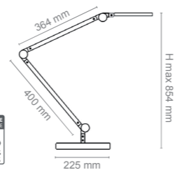
CLELED-0350 Silva LAMPE LED "GIANT" "GIANT" LED LAMP
