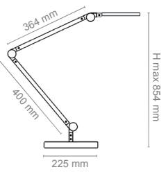
CLED-0350 Silva LAMPE LED "GIANT" "GIANT" LED LAMP
